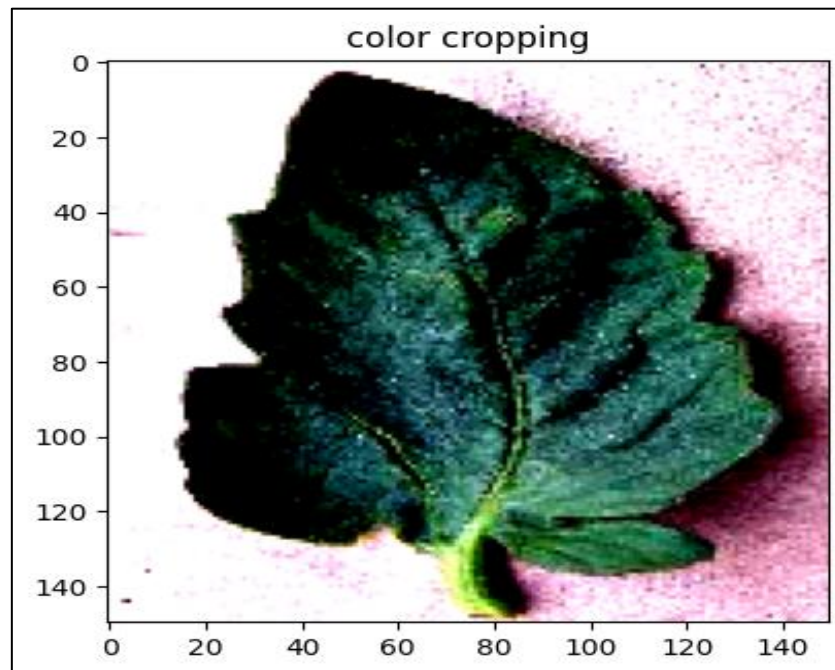
Figure 6 Color Cropping
