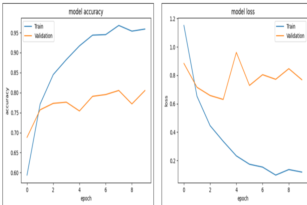
Figure 8 Training Models
