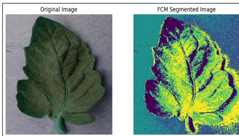
Figure 7 FCM Segmentation
