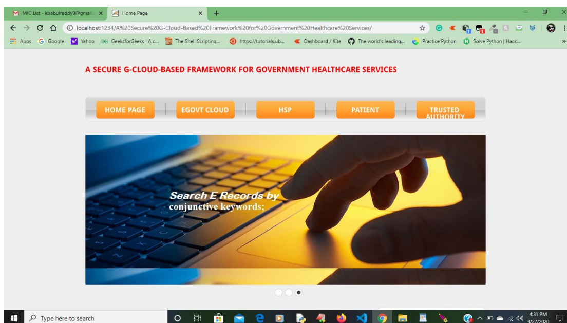
Fig 4.1 Home Page
